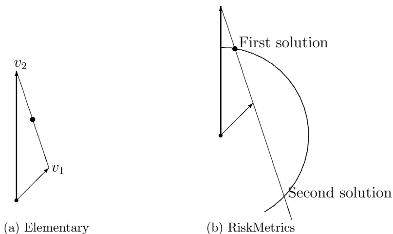
FIGURE 2. Geometrical representation of the elementary and the RiskMetrics mappings
