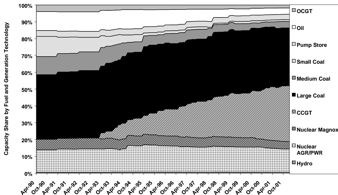
Figure 4: Capacity share by fuel and generation technology 1990–2002
