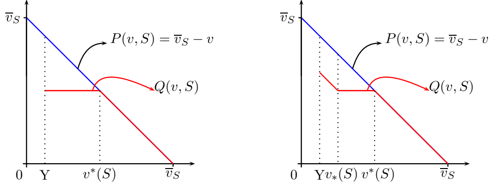
Figure 5: Second-Best Frontier for S \geq \underline{S} .
