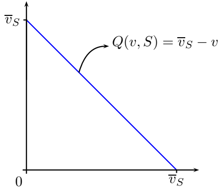
Figure 6: Second-Best Frontier for S < \underline{S} .
