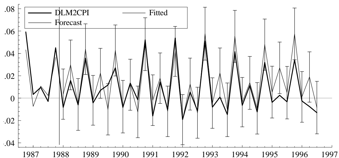
Fig. 6: One-step ahead forecasts of \Delta LM2
