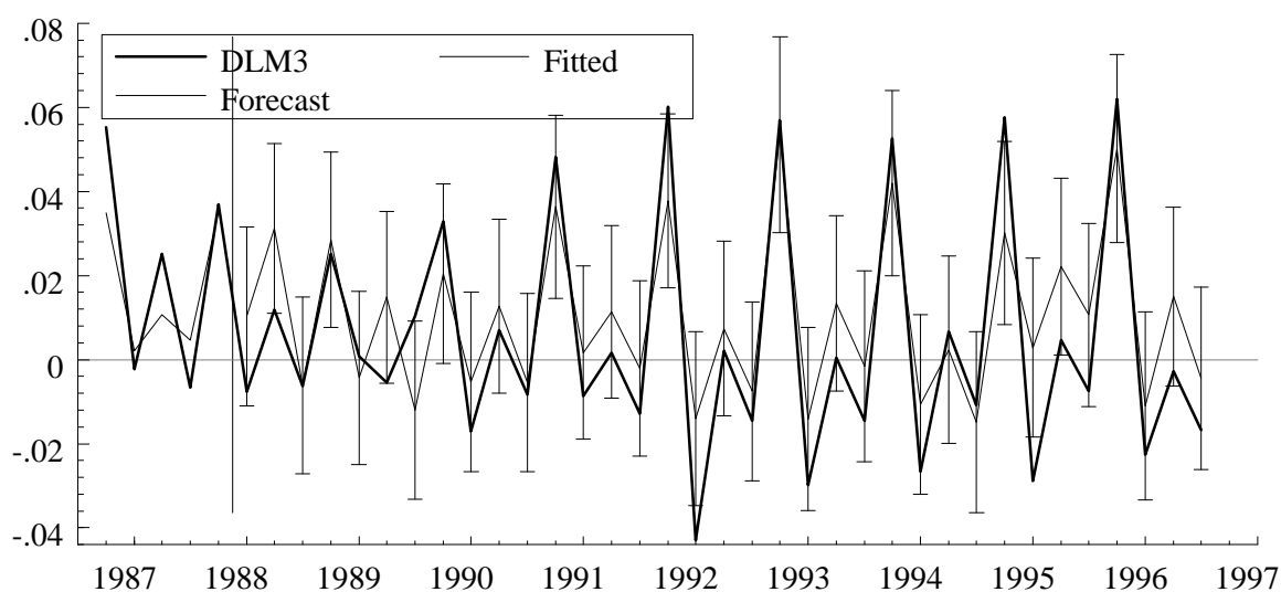
Fig. 9: One-step ahead forecasts of \Delta LM3
