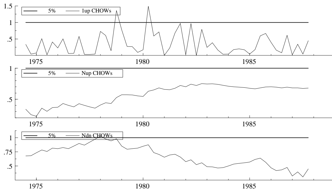
Fig. 1: Recursive Chow-tests of final two-equation model for \Delta LM1
