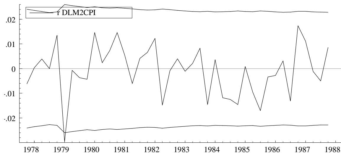
Fig. 5: One-step residuals of \Delta LM2-equation
