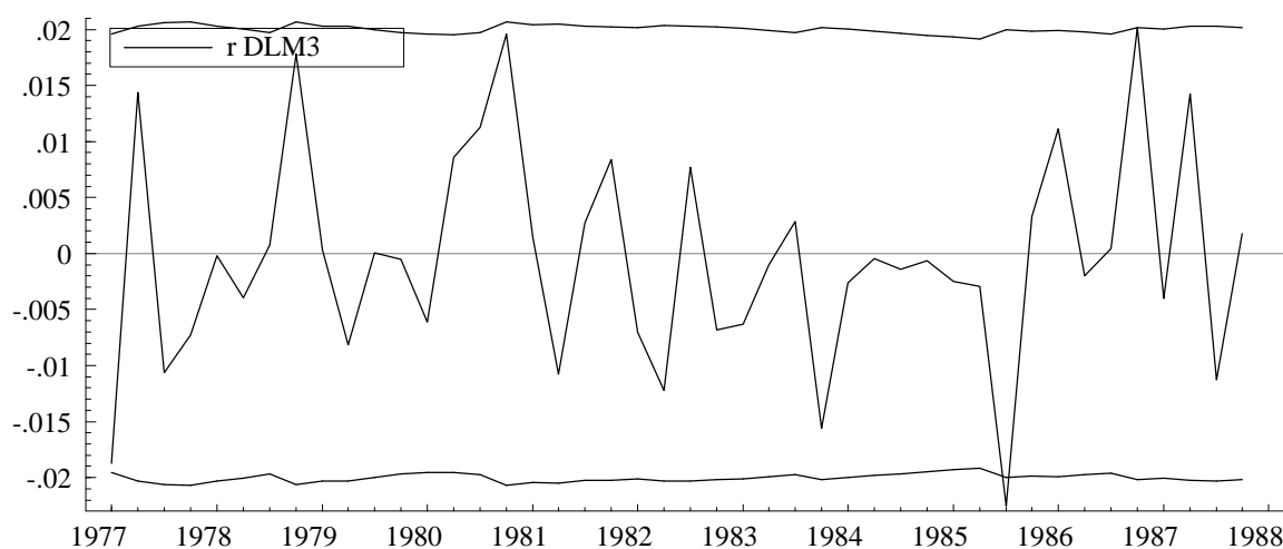
Fig. 8: One-step residuals of \Delta LM3 -equation
