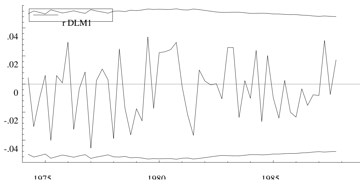
Fig. 2: One-step residuals of \Delta LM1 -equation
