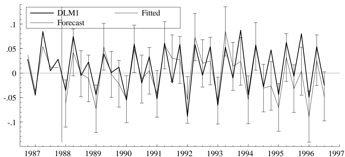
Fig. 3: One-step ahead forecasts of \Delta LM1
