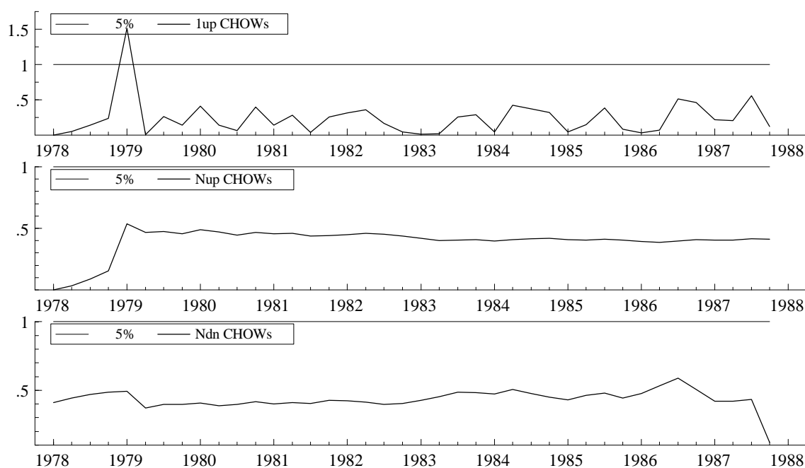
Fig. 4: Recursive Chow-tests of the final two-equation model for \Delta LM2
