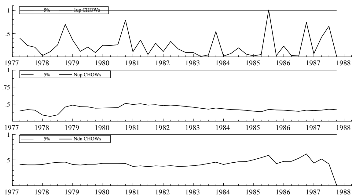
Fig. 7: Recursive Chow-tests of the final two-equation model for \Delta LM3
