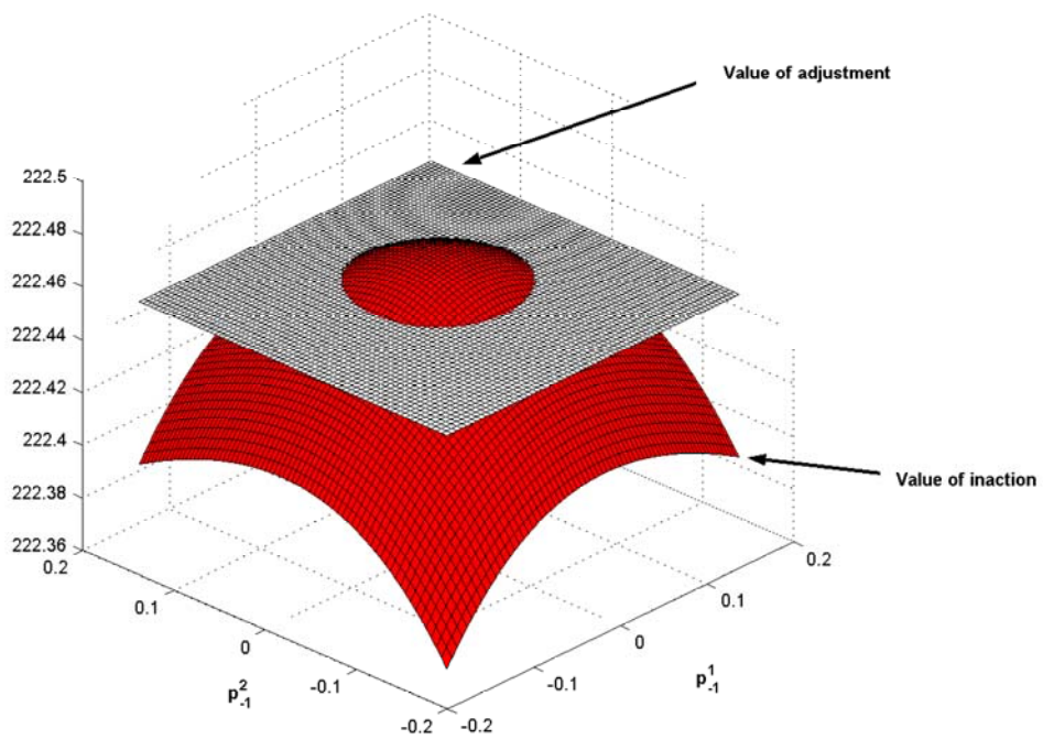
Figure 2: Value Functions
