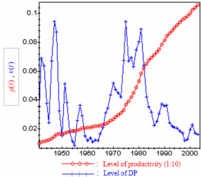
Figure 10 The curves of US economic productivity \mu(t) (GDP (chained) price index; Fiscal Year 2000 = 1,000.) and DP(Development Power) in the time field from 1941 to 2003. The proportion of the real indexes of \mu(t) to drawn indexes is 1:10. Though productivity \mu(t) has been growing approximately, DP fluctuates always.
