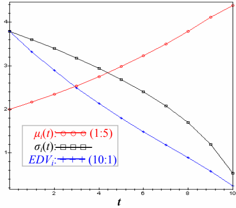
Figure7. The indexes varying process of growth processes with EDP release
