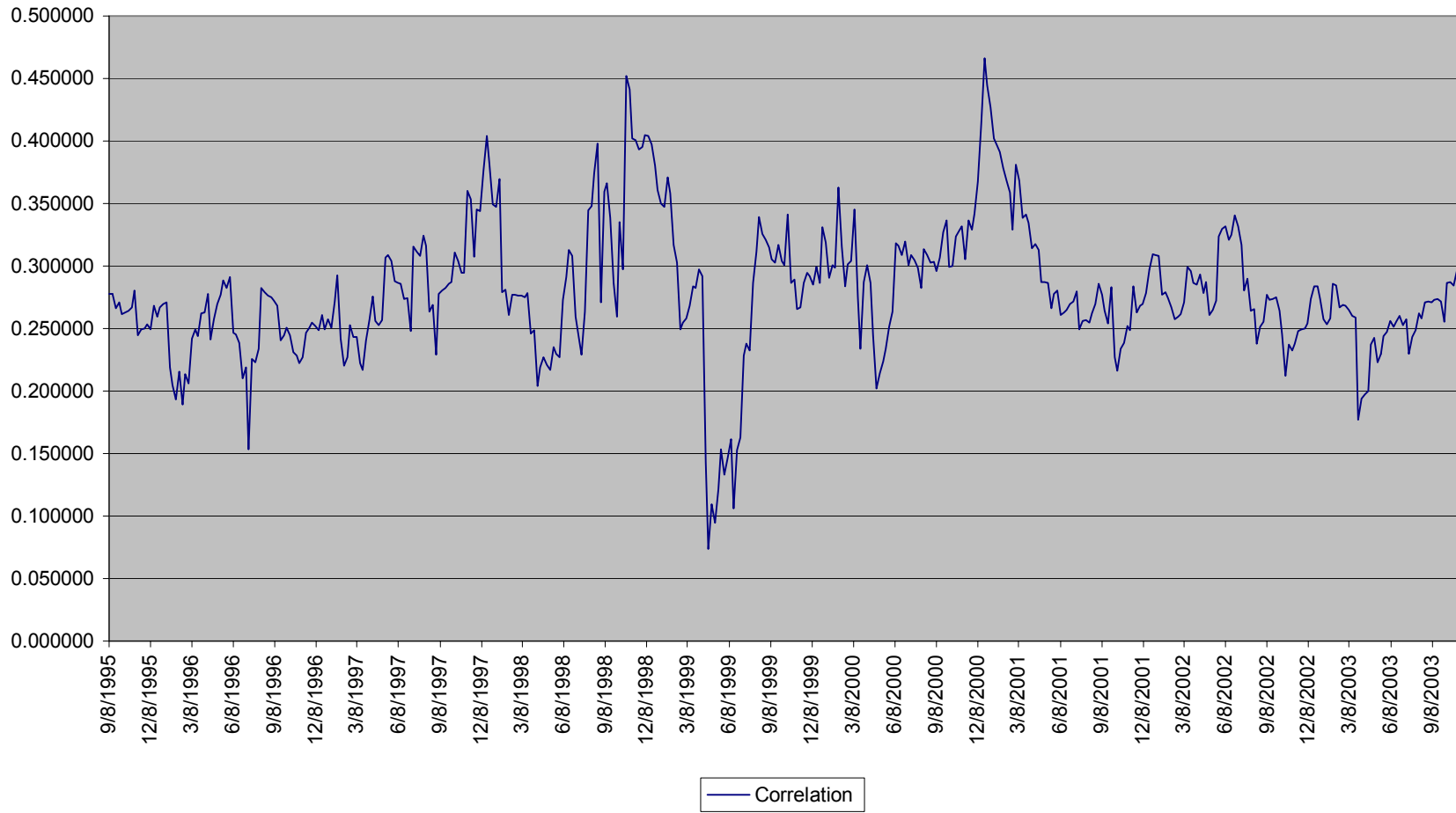
Figure 1: Correlation of RTS Index with S&P 500 Index
