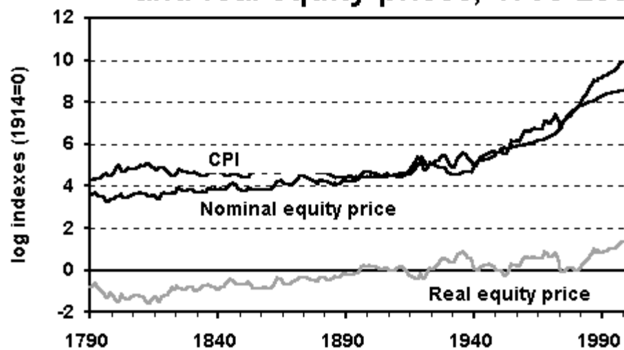
Fig. 4. UK consumer prices, nominal and real equity prices, 1790-2000
