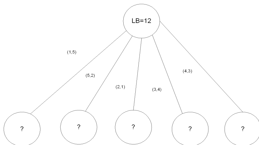
Figure 3.66: A branch and bound tree
