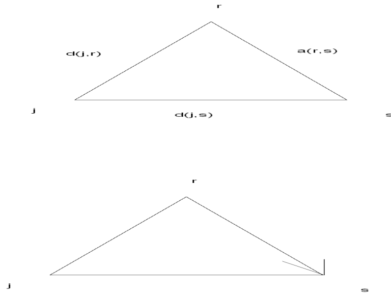
Figure 3.93: Vertex-Arc distance.
