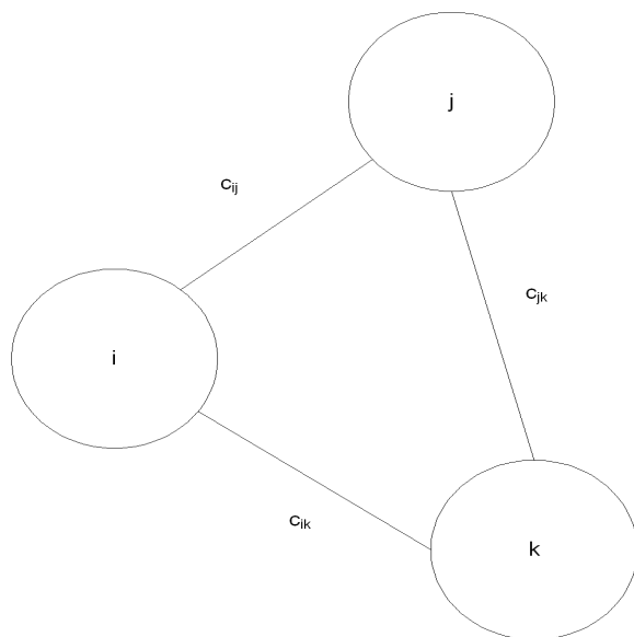
Figure 3.70: Cheapest insertion heuristic.
