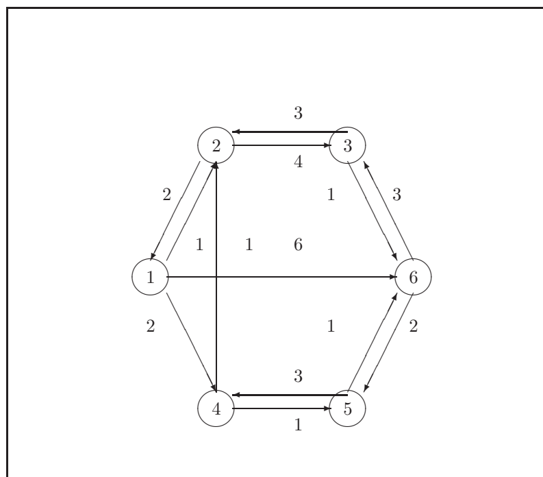
Figure 3.59: A Network
