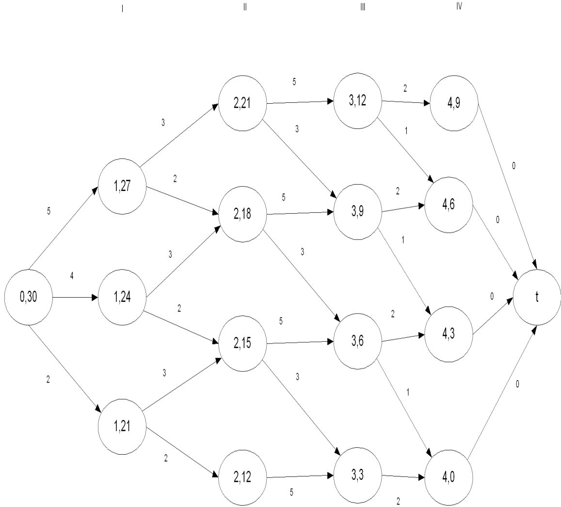
Figure 3.60: The network showing the 4 phases of the problem.
