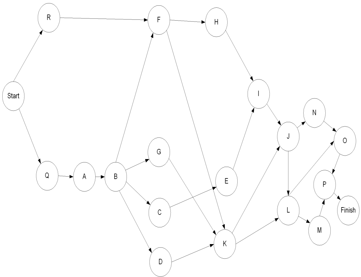
Figure 3.48: The pipe line example with activities on the nodes.
