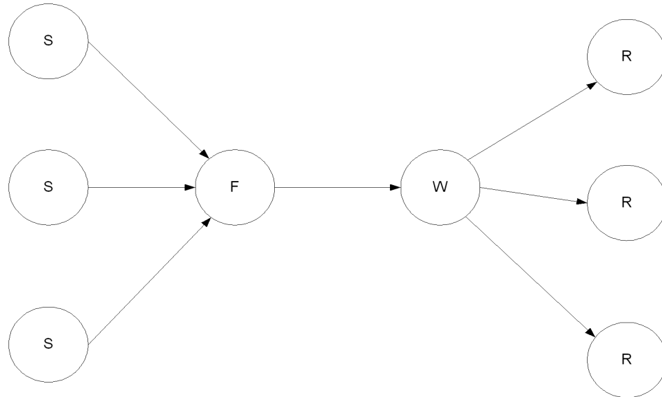
Figure 3.89: Warehouse example.
