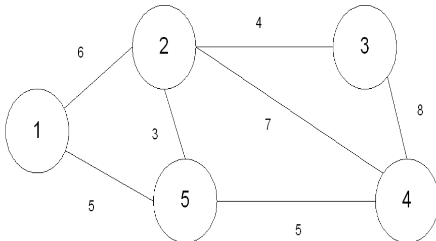
Figure 3.19: An example of a maximum capacity route.
