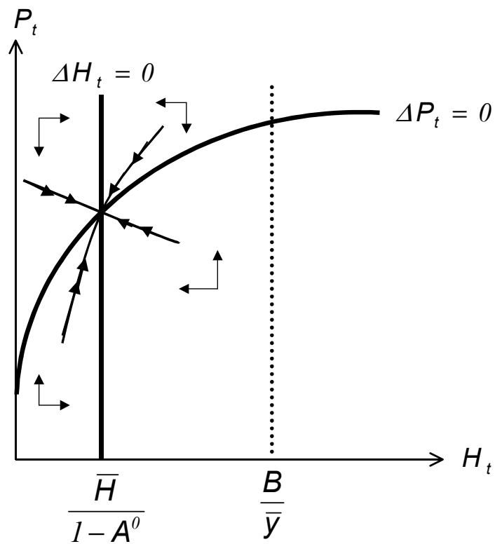
Figure 4.1: The phase diagram.
