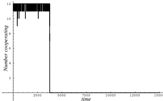
Fig. 5. Outbreak of defection. At t = 0 , two cooperating groups of size n = 6 merge to form a larger, cooperating group of size n = 12 . The agents follow bandwagon expectations and have horizon length H = 9.5 throughout, with p = 0.93 , b = 2.5 , c = 1 , \alpha = 1 and \tau = 1 . For these parameters, cooperation is the optimal state for a group of size n = 6 , but for the combined group of size n = 12 , cooperation is metastable. Indeed, as the figure shows, metastable cooperation persists for almost 4,000 time steps in this example. Uncertainty ( p less than one) ensures that eventually a large fluctuation in the perceived number of agents cooperating eventually takes the group over into a state of mutual defection, which is optimal.
