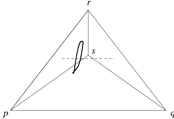
FIGURE 1. The oscillating attractor for \varepsilon = 0.2 .
