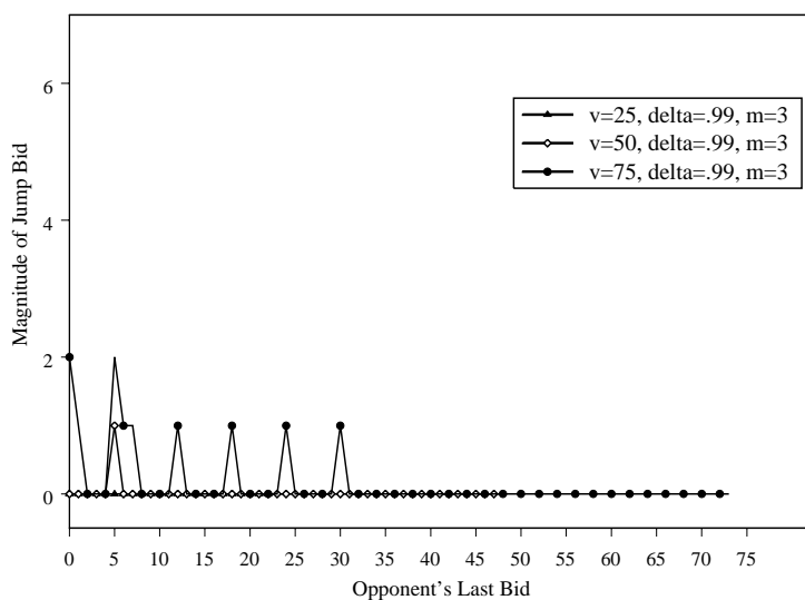
Figure 3: Portion of equilibrium bids that are above minimum increment assuming the values are uniformly distributed, \delta = .99 and m = 3 .
