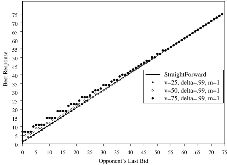
Figure 1: Depiction of complete equilibrium strategies for bidders with values of 25, 50 and 75 assuming values are uniformly distributed, \delta = .99 and m = 1 .
