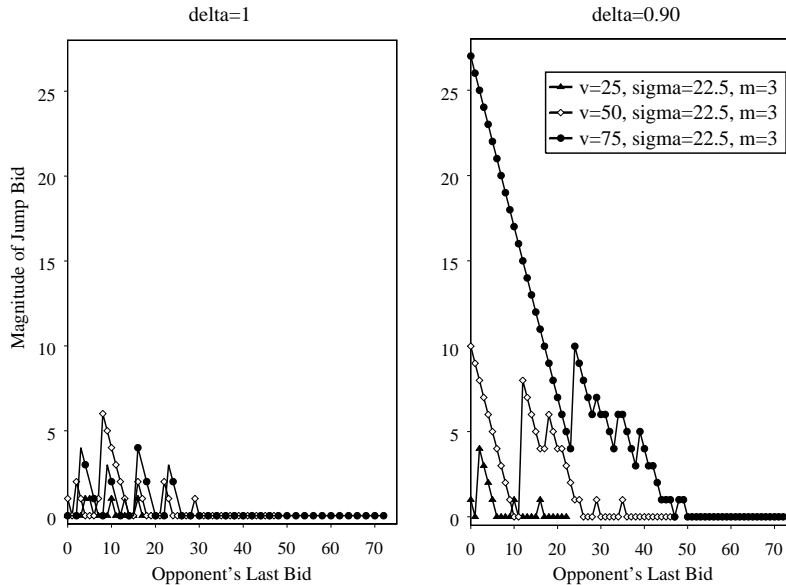
Figure 4: Comparison of equilibrium bidding strategies between \delta = 1 and \delta = .9 assuming normally distributed values, \sigma = 22.5 , m = 3 .
