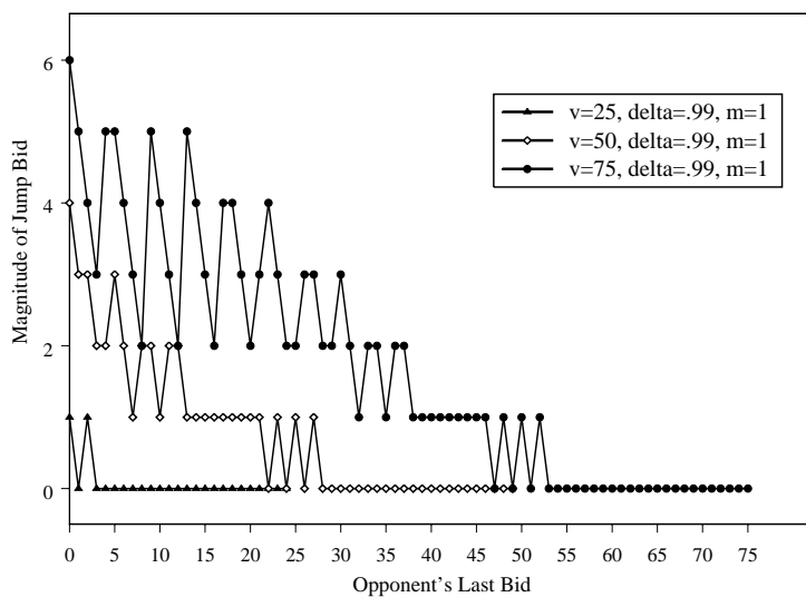
Figure 2: Portion of equilibrium bids that are above minimum increment assuming the values are uniformly distributed, \delta = .99 and m = 1 .
