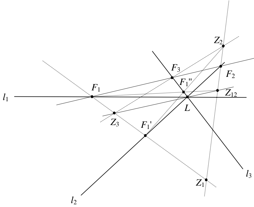
Fig. 4 The case k = 3 for Lemma 3.
