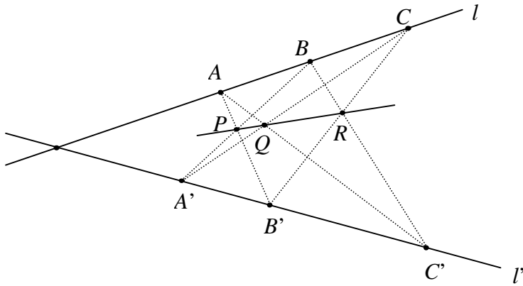
Fig. 1 Pappus' theorem.
