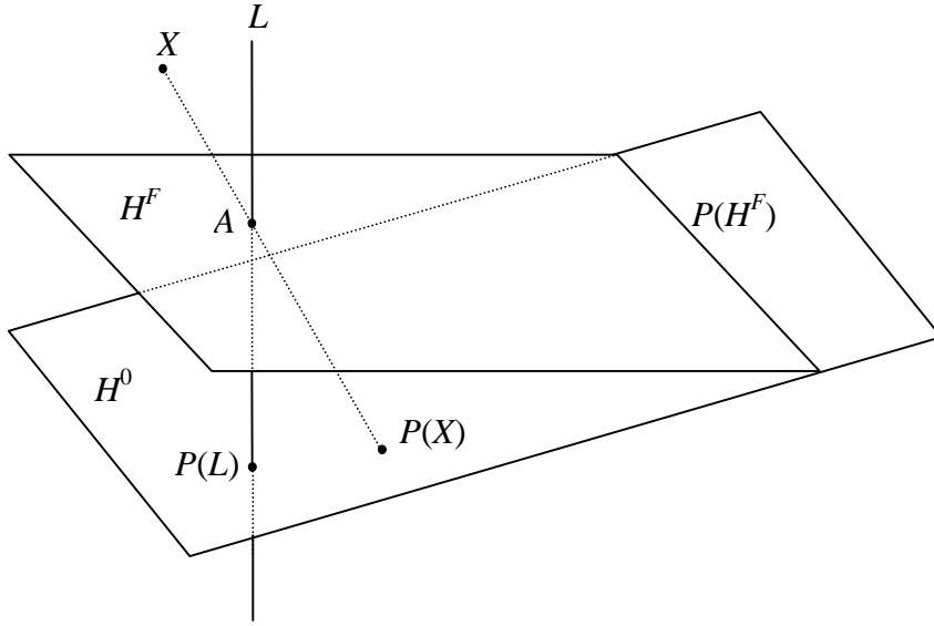
Fig. 5 Configuration in the proof of Theorem 2 for n = 3 and k = 4 .
