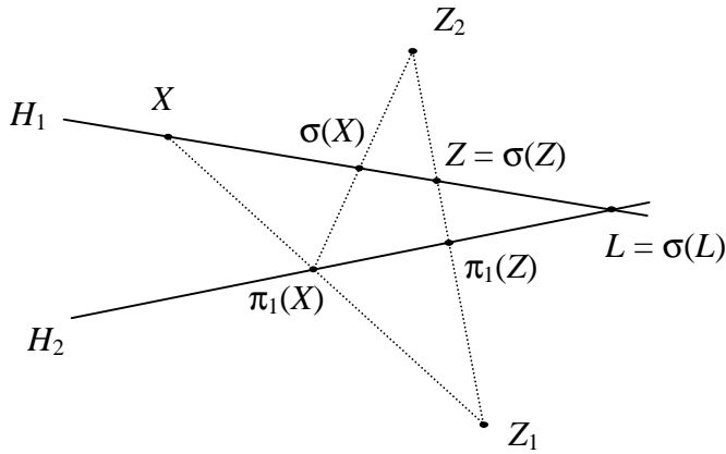
Fig. 2 The axis L and the center Z of a perspective collineation composed of two perspectivities in P^2(\mathbf{R}) .
