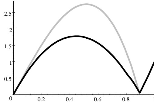
Figure 2: Admissible values of \sigma and \delta in the OPM cycle example.
