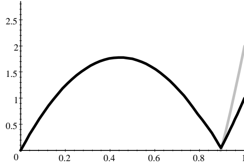
Figure 3: Admissible values of \sigma and \delta in the TPM cycle example.
