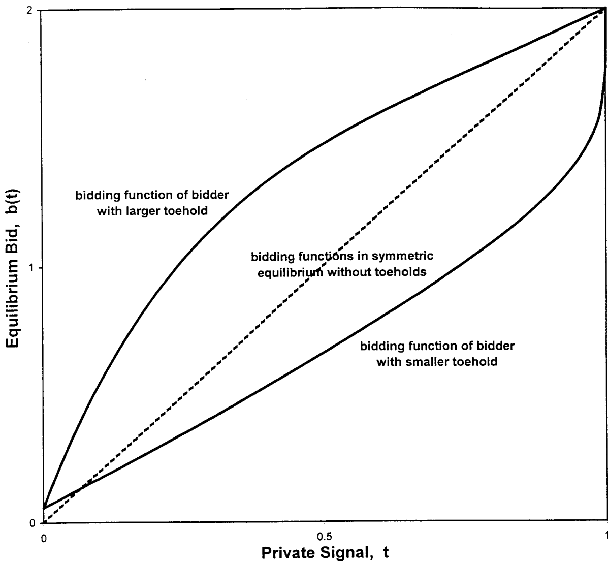
Figure 1: Equilibrium Bidding Functions With and Without Toeholds for Linear Example v = t_1 + t_2 .
