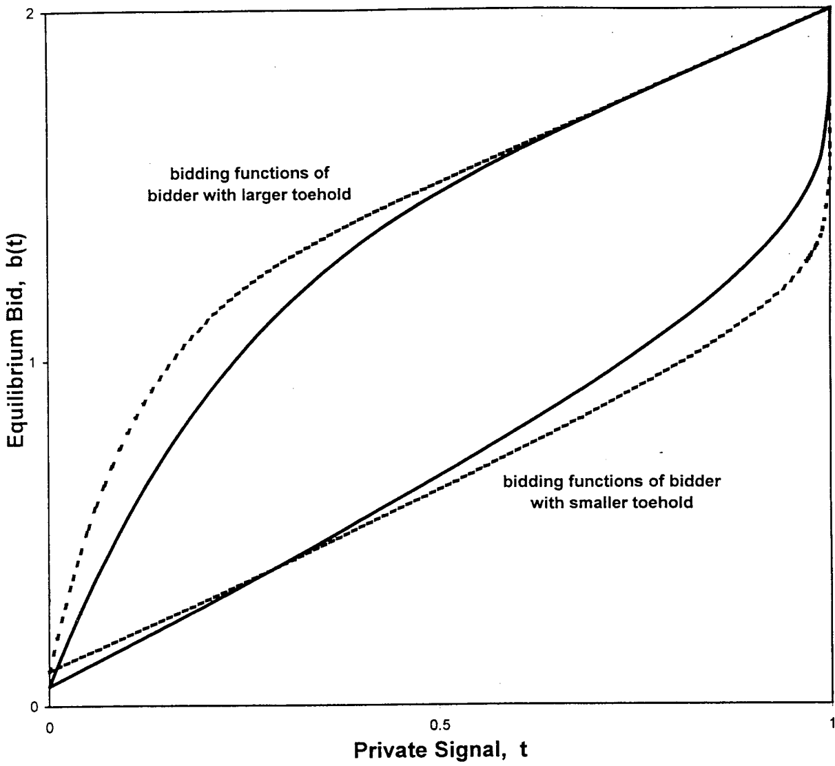
Figure 2: Equilibrium Bidding Functions With Different Size Toeholds for Linear Example v = t_1 + t_2 .
