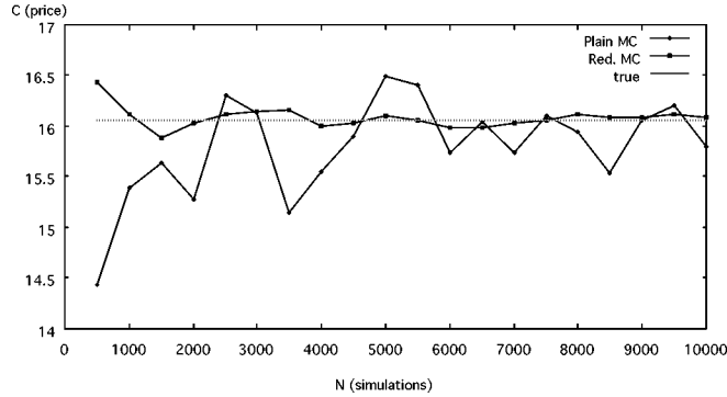
Figure 1: Estimates of exchange option price with plain and variance reduction Monte Carlo.
