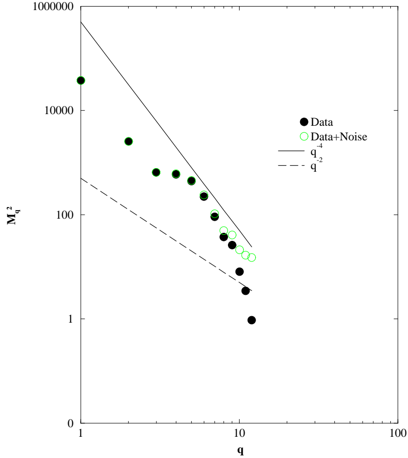
Figure 5: The eigenvalues M_q^2 of the instantaneous fluctuation matrix M(\theta, \theta') , as a function of their rank q = 1, 2, \dots , in log-log coordinates. We have shown for comparison a q^{-2} and a q^{-4} decay (see section 5), indicating that these eigenvalues are decreasing very fast with q . Also shown for comparison the eigenvalues of M(\theta, \theta') when an artificial noise (uniform in [-0.02, +0.02] ) is independently added to each point of the FRC, to estimate the relevance of the information contained in the high q eigenvalues.
