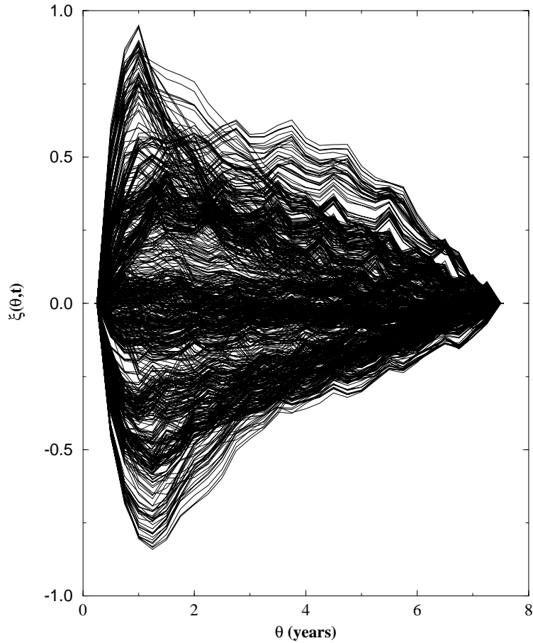
Figure 3: This shows the deviation \xi(t, \theta) as a function of \theta for different times t . Note that this resembles the motion of an elastic string, with a maximum around \theta = 1 year.
