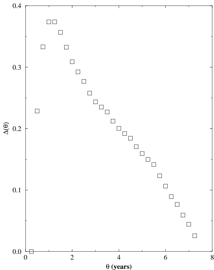
Figure 4: Root mean square deviation \Delta(\theta) from the average FRC as a function of \theta . Note the maximum for \theta^* = 1 year, for which \Delta \simeq 0.38\% .
