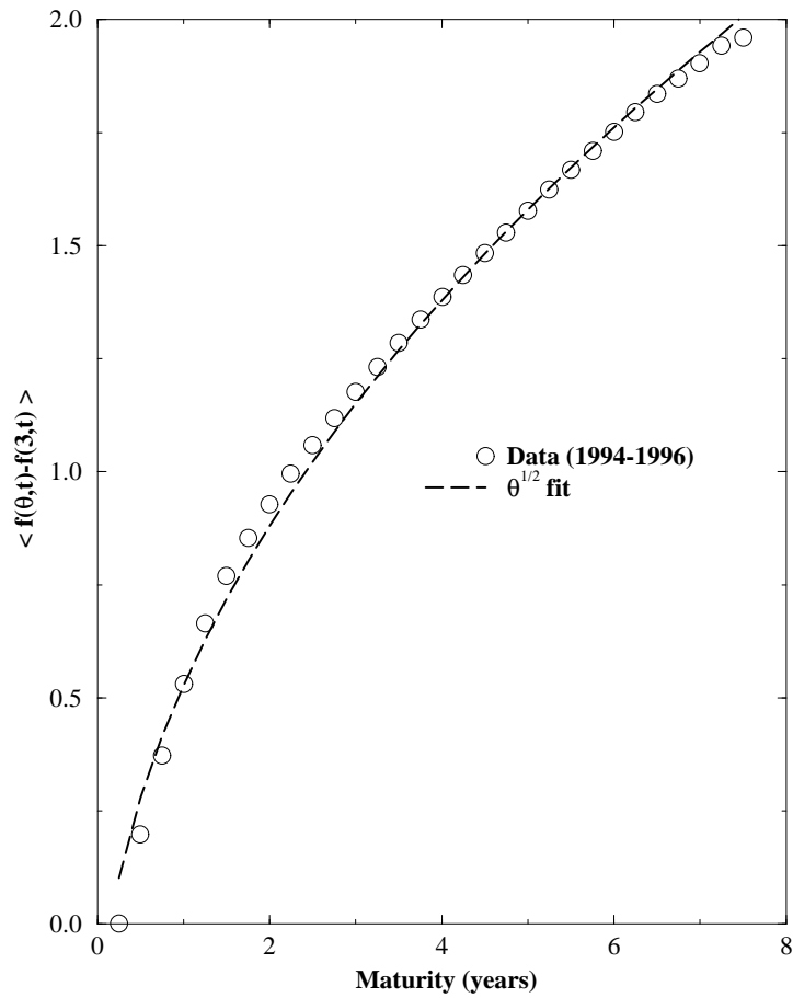
Figure 2: The average FRC in the period 94-96, as a function of the maturity \theta . We have shown for comparison a one parameter fit with a square-root law, A(\sqrt{\theta} - \sqrt{\theta_{\min}}) . The same \sqrt{\theta} behaviour actually extends up to \theta_{\max} = 10 years, which is available in the second half of the time period.
