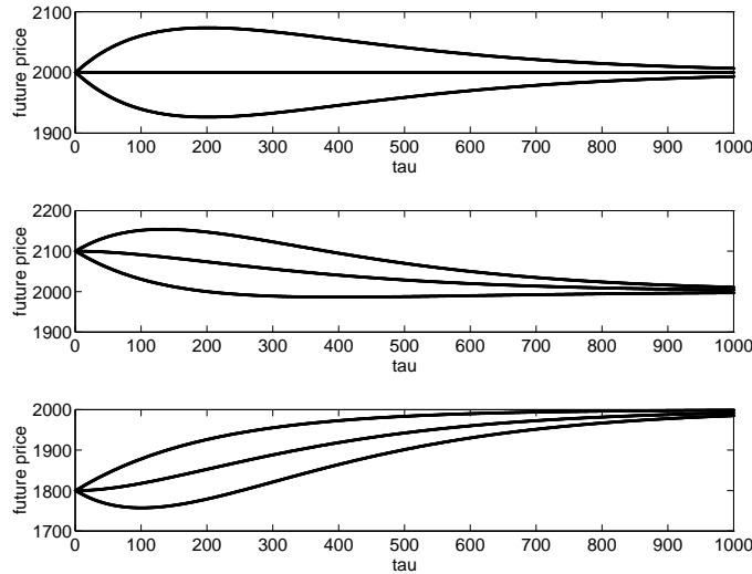
Fig. 1. Expectations of individuals about future price movements given by integrating eqn. 6 for the case in which \sigma = 0 and H_t = 200 . Fundamental valuation p_f is set at 2000. The three cases show the expectations when the current market price, p'(t + \tau)_{\tau=0} = p(t) is set at 2000 (upper figure), 2100 (middle figure), and 1800 (lower figure). For each figure, the three curves represent the trends, T(t) given by +1, 0, and -1.
