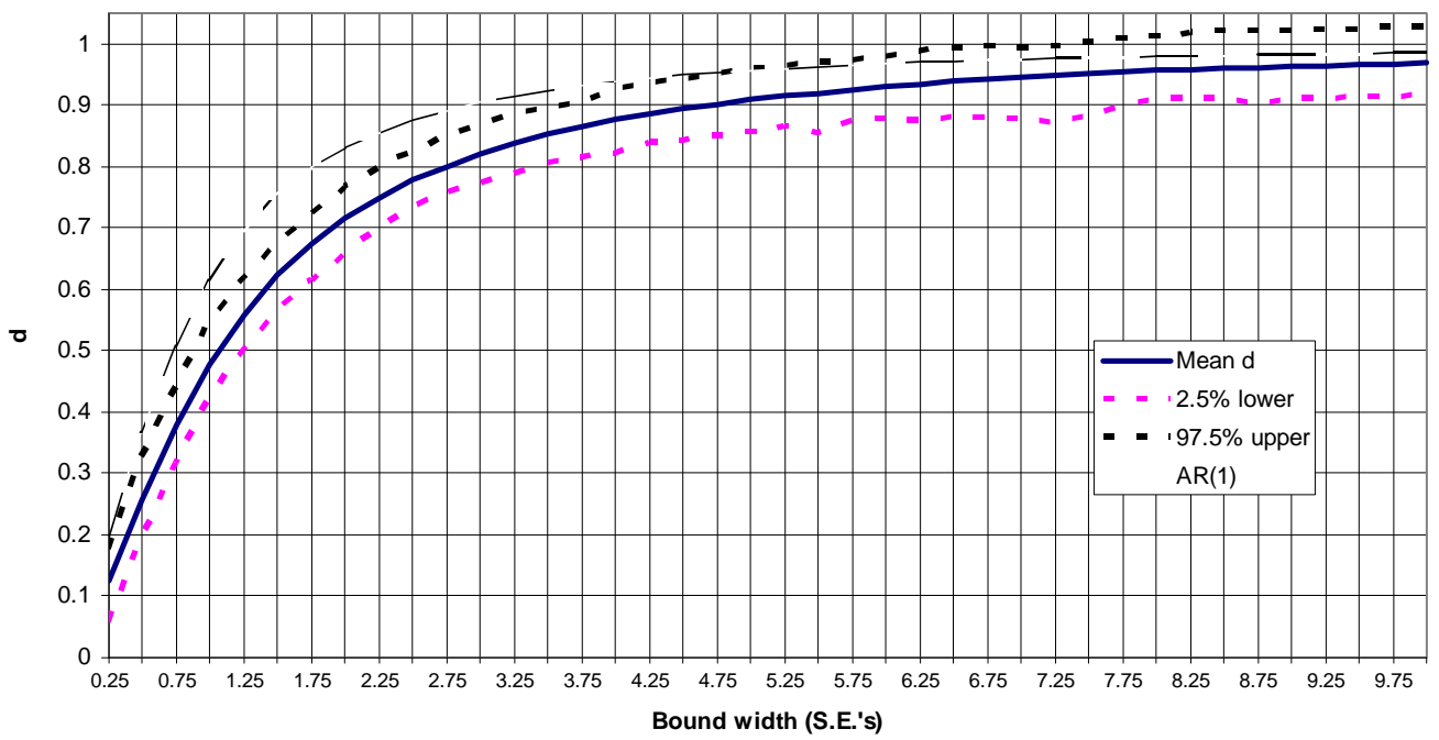
Figure 1: SIMULATIONS OF d FROM EQUATION (2) 1000 Simulations at Each Bound
