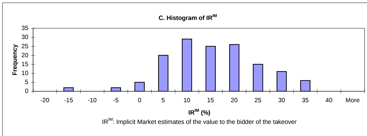
Fig. 5. Histograms of value improvement measures. Sample includes 1018 tender offers where both bidder and target were listed on the NYSE, AMEX, or NASDAQ during 1962-2001; additionally, for IR^{IM} the sample is restricted to cases where there was a competing bid for the target.
