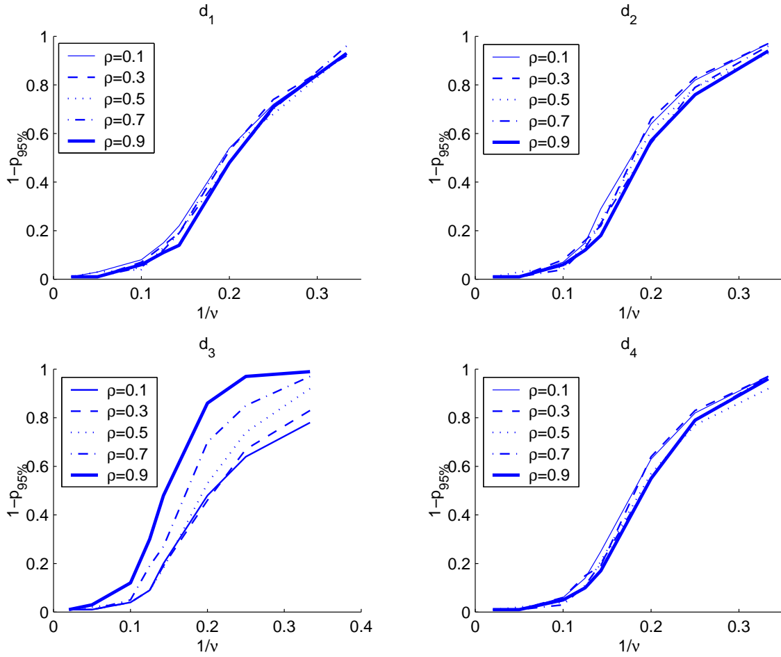
Figure 5: Graph of the minimum significance level ( 1 - p_{95\%} ) necessary to distinguish the Gaussian copula hypothesis H_0 from the hypothesis of a student copula with \nu degrees of freedom, as a function of 1/\nu , for a given distance d_i and various correlation coefficients \rho = 0.1, 0.3, 0.5, 0.7 and 0.9 .
