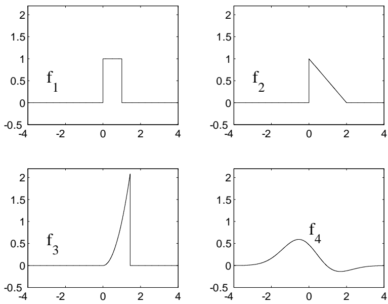
Figure 2: Graphs of the nonlinear functions f used in DGPs
