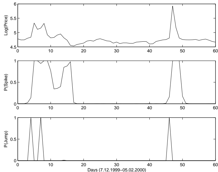
Fig. 2. The deseasonalized log-spot price d_t since December 7, 1999 until February 5, 2000 ( top panel ) together with the probability of being in the spike regime for the estimated two-regime model with lognormal spikes ( middle panel ) and of being in the jump regime for the estimated three-regime model ( bottom panel ).
