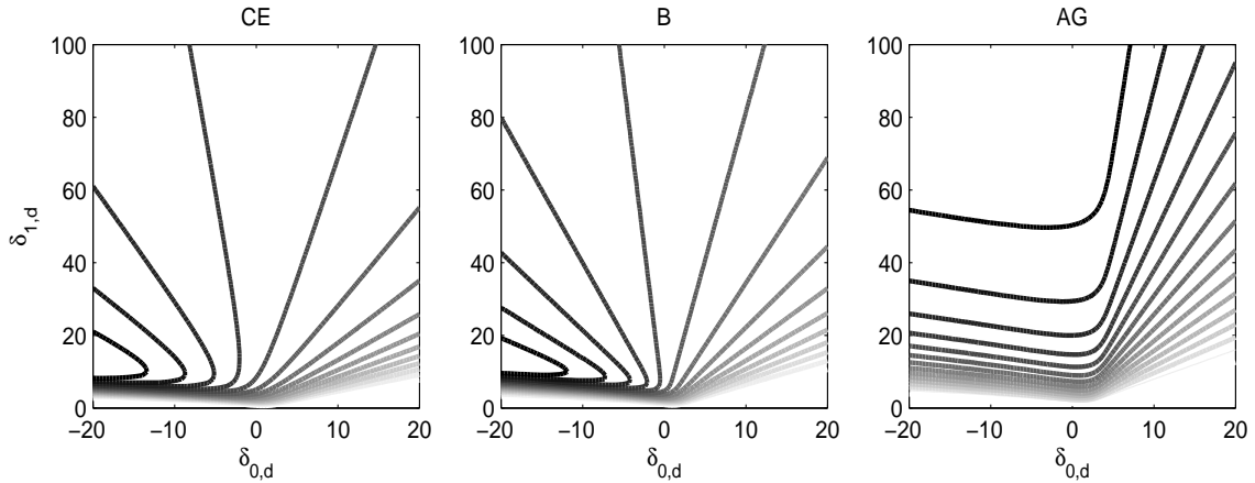
Figure 2: Contour plots of the measures are univariate skewness for varying \delta_{0,d} and \delta_{1,d} . Darker contours indicate larger values of skewness.
