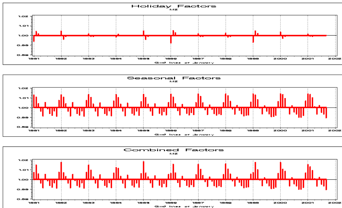
Figure 16: Holiday, Seasonal and Combined Factors for M2
