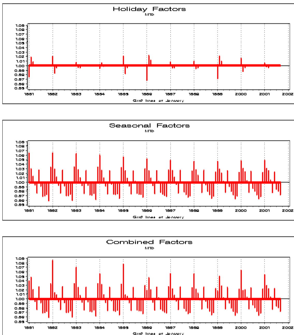
Figure 15: Holiday, Seasonal and Combined Factors for M1b
