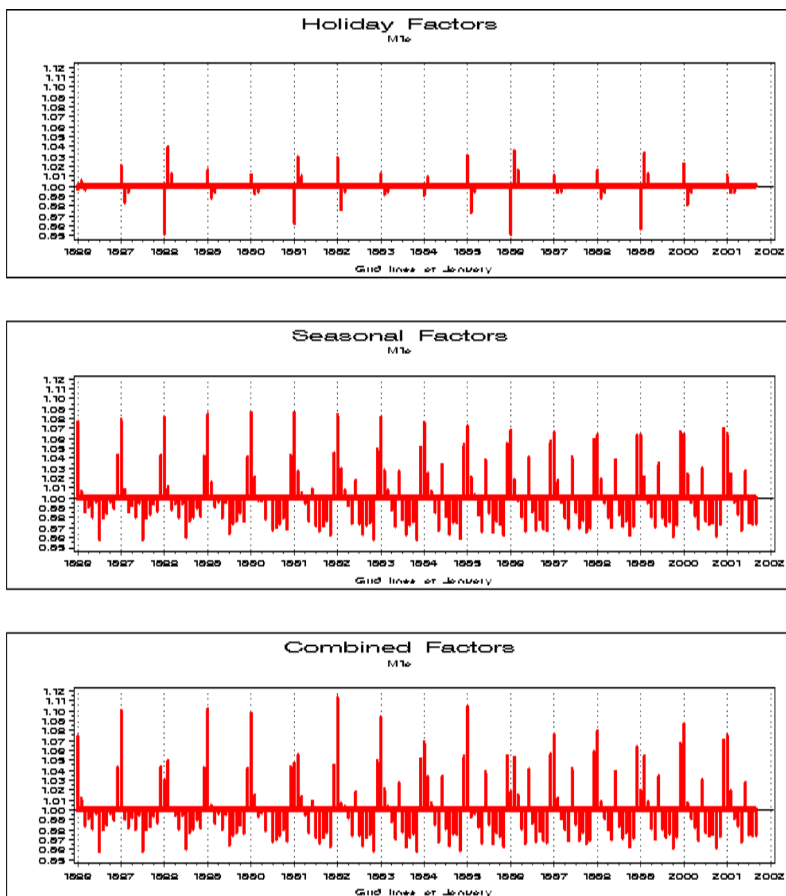
Figure 14: Holiday, Seasonal and Combined Factors for M1A
